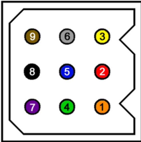
9-pin Molex Wiring Diagram (rear panel view)
